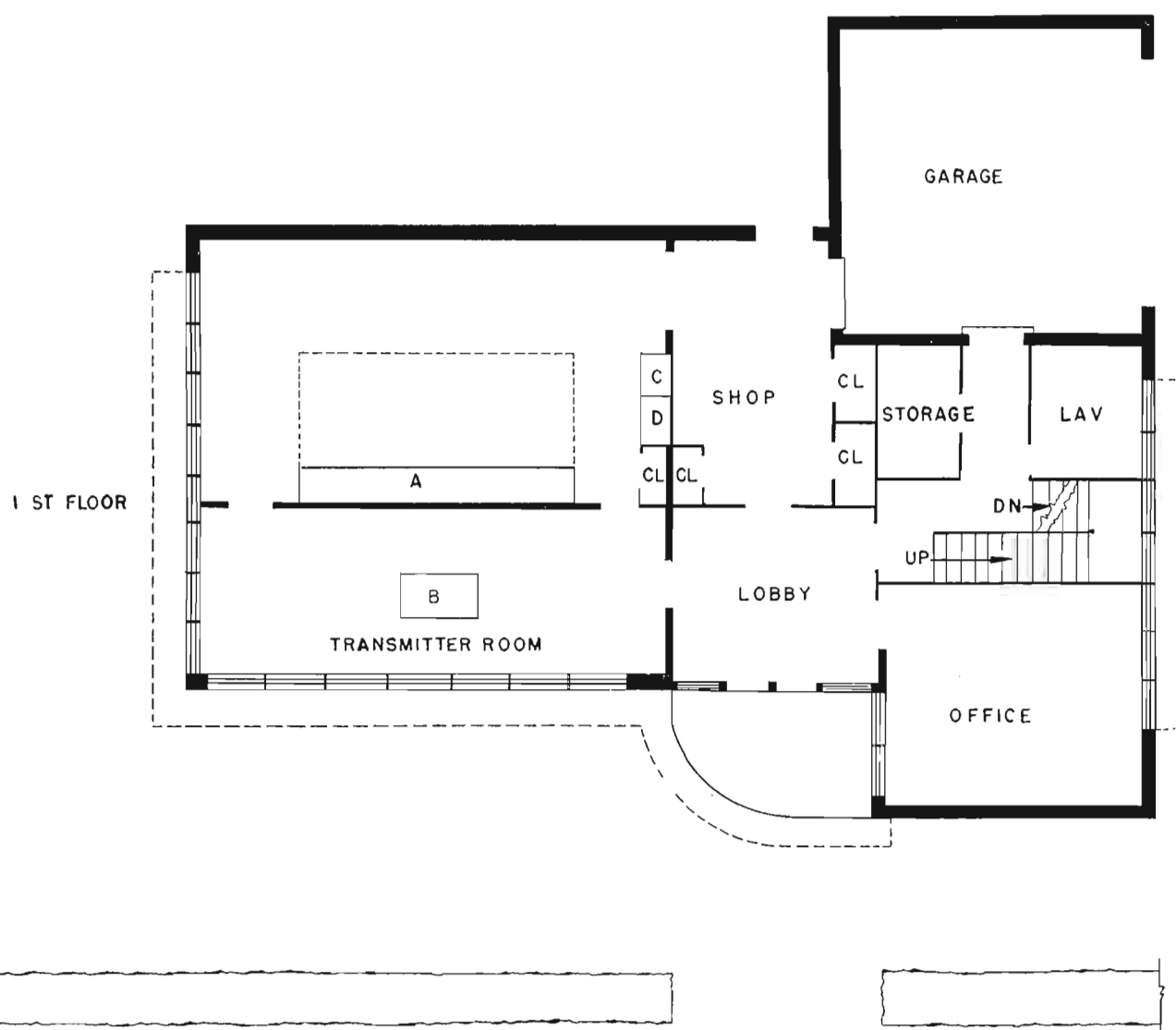
SUGGESTED TRANSMITTER BUILDING FOR 50 KW FM
