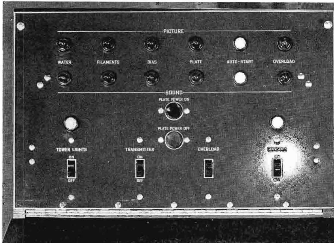
FIG. 17. Left-hand control panel. Start-stop controls, tower lights, etc., plus signal lights indicating operating status are mounted on this panel.
