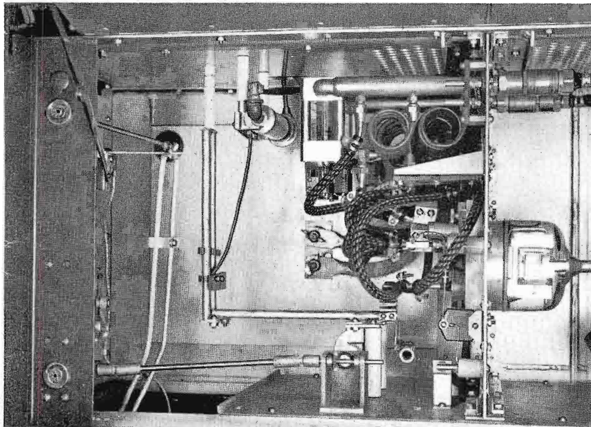
FIG. 5. (above) Power amplifier section of the picture transmitter showing method of mounting 8D21 tube. The grid tank circuit shown in this view is a quarter wave line (three quarter wave for channels 7 to 13). The plate tank circuit of this amplifier is similar to that of sound p.a. shown on page 10.
