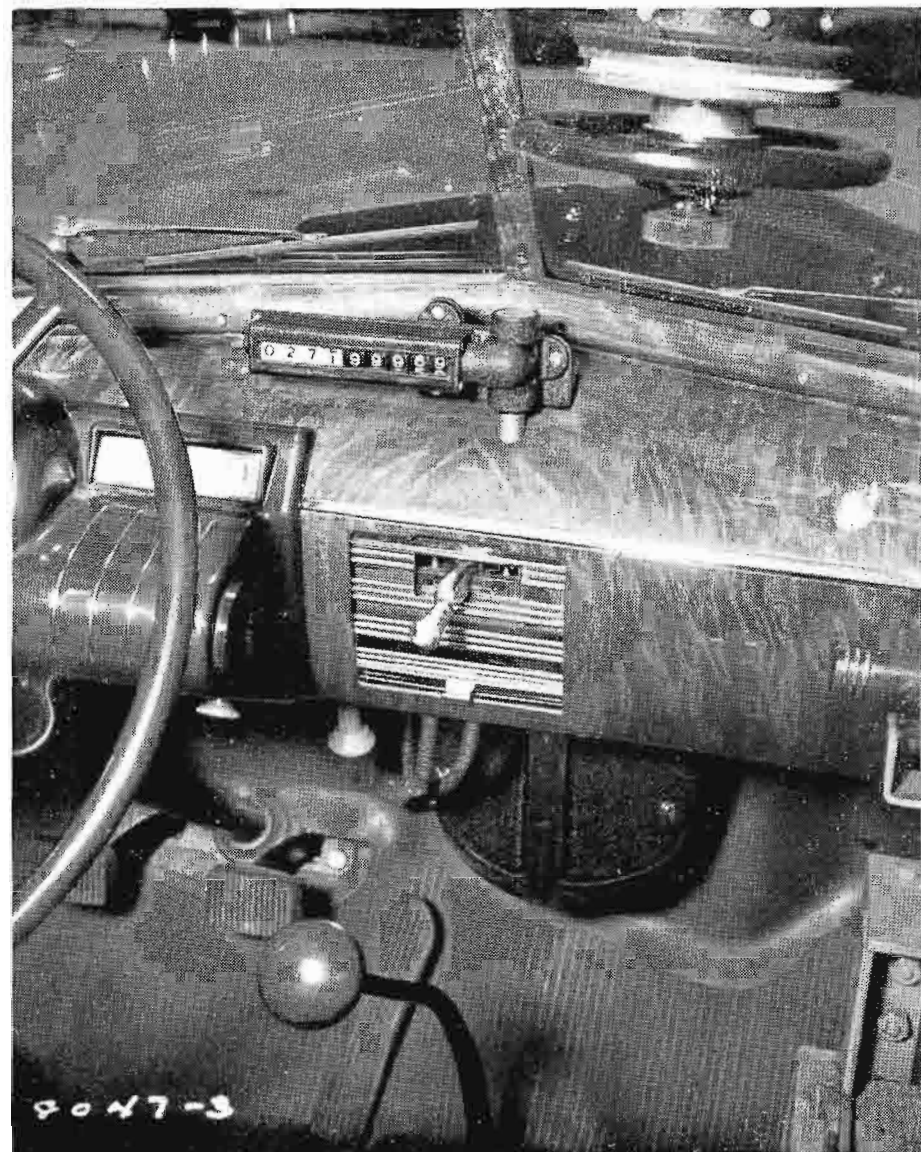
FIG. 13. In order to coordinate recorder readings with the location of the car, the recorder chart mechanism is geared to the speedometer drive shaft. Clutch is shown in this view.
