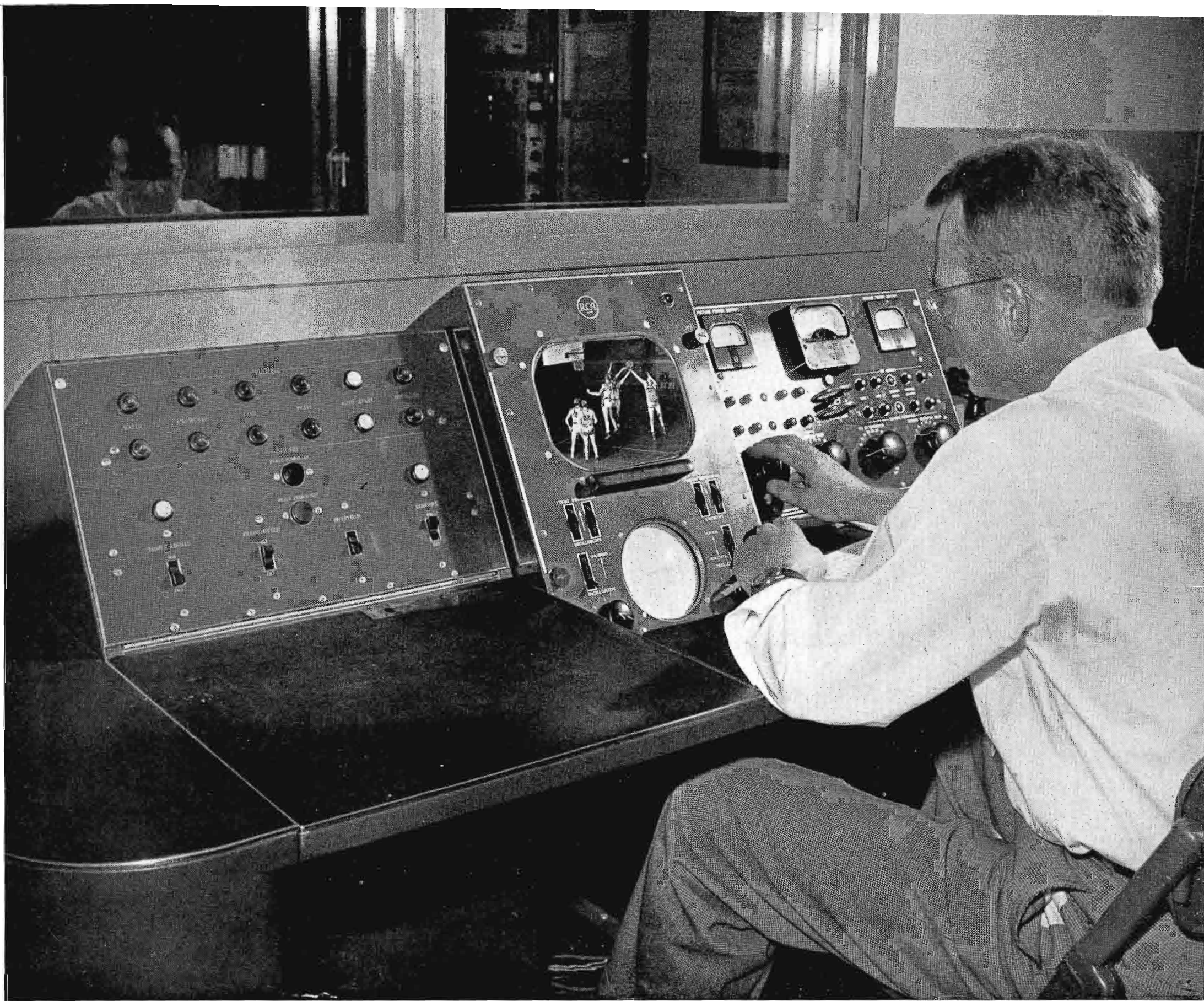
FIG. 4. Transmitter control console at WTMJ-TV. The transmitter operator, seated at the console, has complete finger-tip control of the RCA TT-5A transmitter which may be seen through the window. Complete sound and picture control and monitoring is provided.
