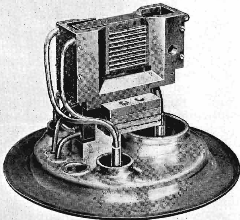
HEADER WITH FILAMENT, GRID № 1, AND GRID № 2 IN POSITION
