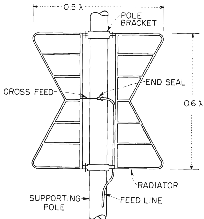
FIG. 2. One pair of Superturnstile radiators mounted on steel pole. Other pair is at right angles to these, using same pole brackets.
