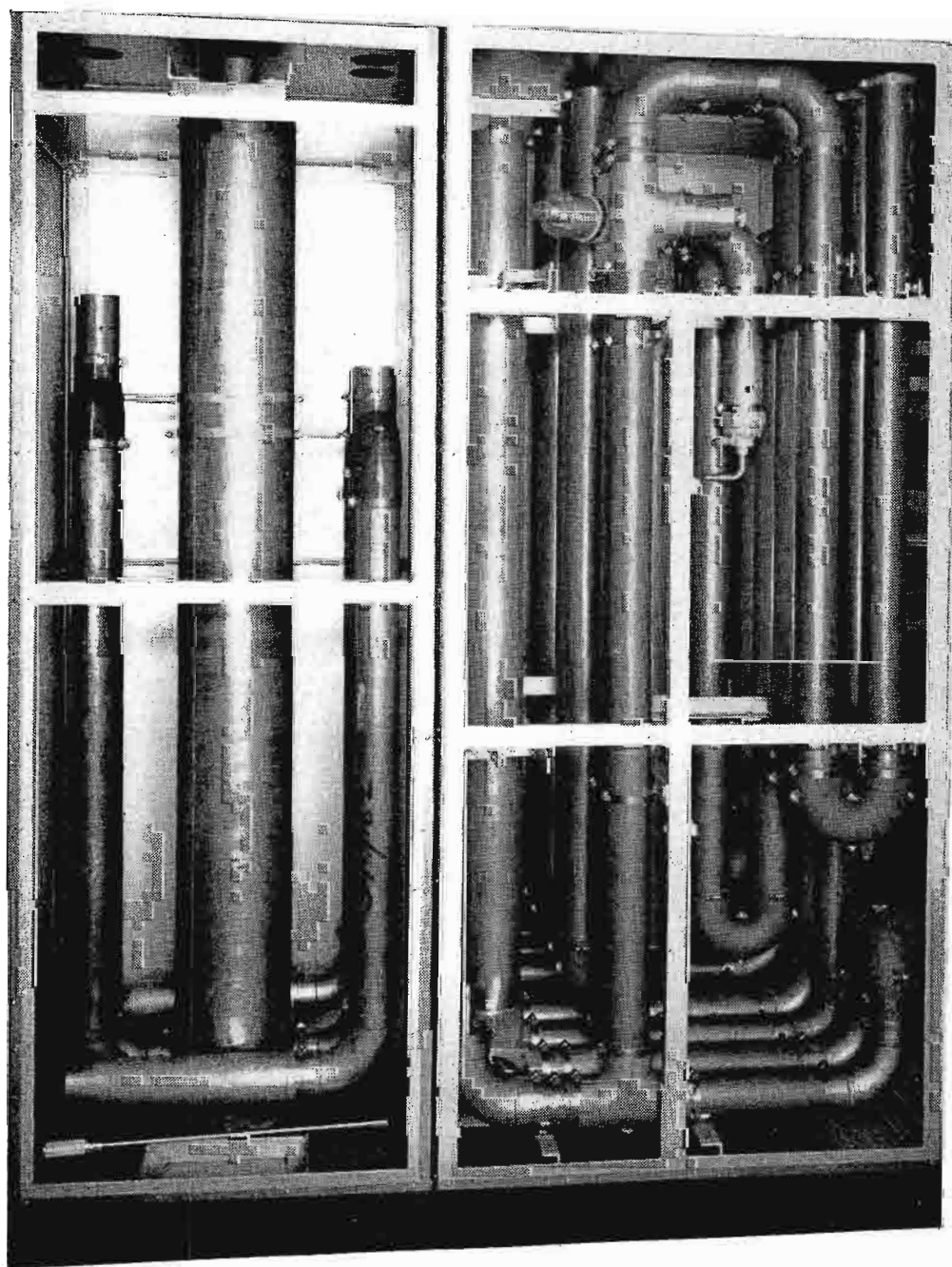
FIG. 15. Duplexer (left) and sideband filter (right) with sides removed to show the folded back coaxial lines which make up the capacitances and inductances used (see diagram Figure 12).
