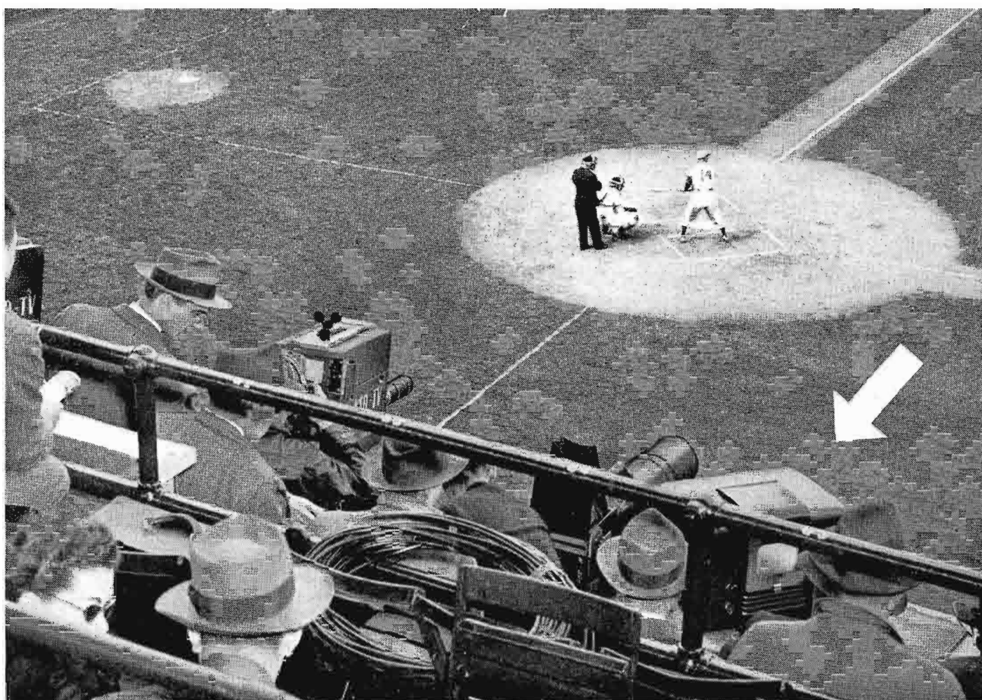
FIG. 2. (Right, upper)—Arrow points to a converted seven-inch screen television receiver (RCA Model 621 TS) used as a monitor for the KSD-TV sport telecast announcer at Sportsman's Park, home of the St. Louis Cardinals and Browns. With "one eye" on the monitor the announcer can be assured that any action or unusual play he describes is in the angular field of the camera.
