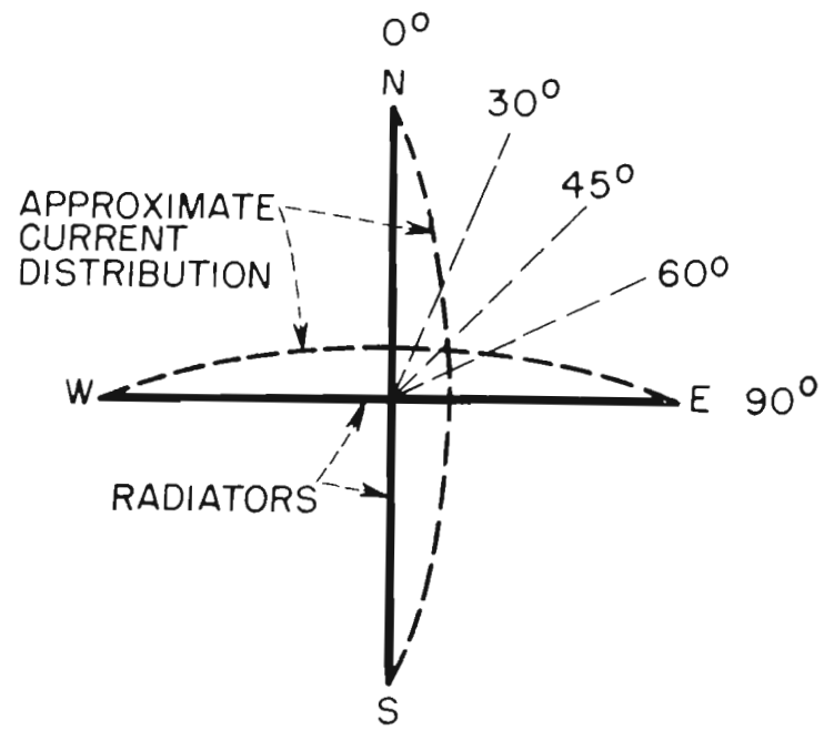
FIG. 1. (above) Horizontal plane through radiators connected in turnstile arrangement.
