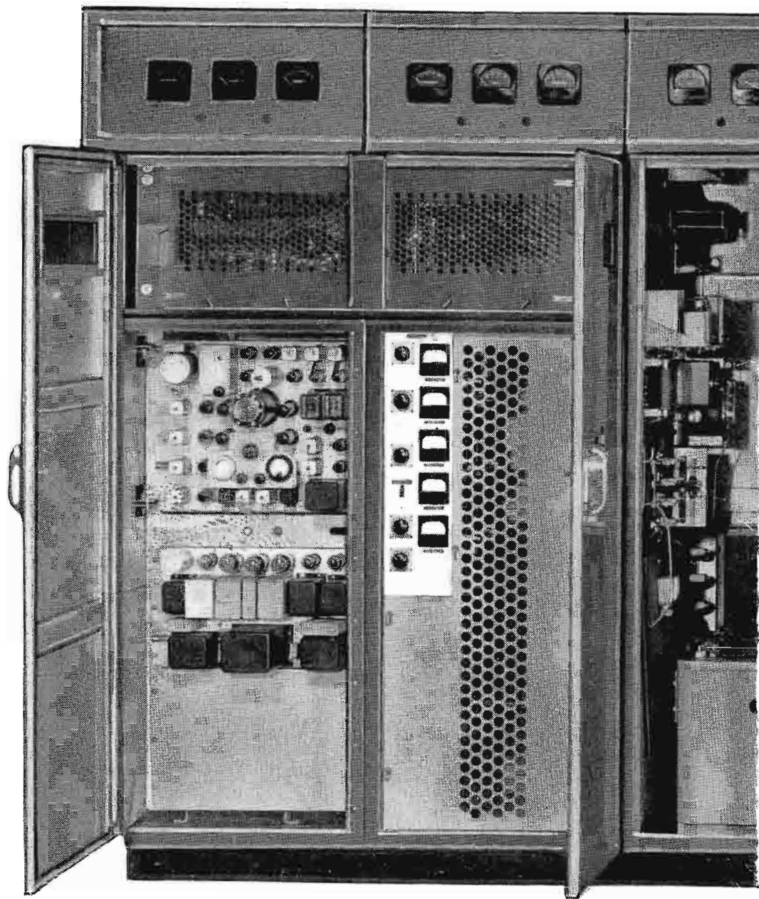
FIG. 1. TT-5A Transmitter with front doors open to show accessibility. Frames 1 and 2 house the sound transmitter; frame 3, the
