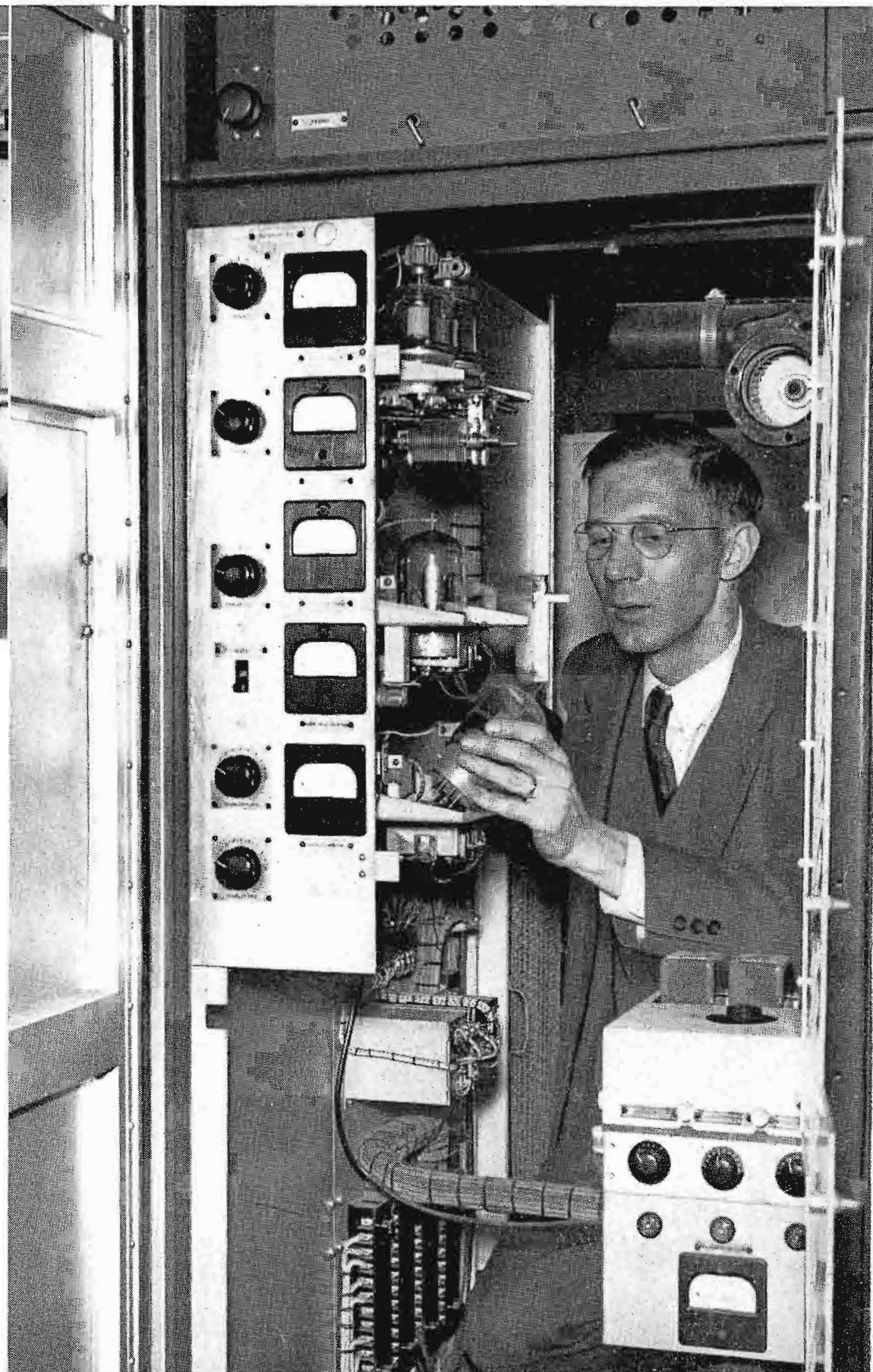
FIG. 5. (above) Power amplifier section of the picture transmitter showing method of mounting 8D21 tube. The grid tank circuit shown in this view is a quarter wave line (three quarter wave for channels 7 to 13). The plate tank circuit of this amplifier is similar to that of sound p.a. shown on page 10.
