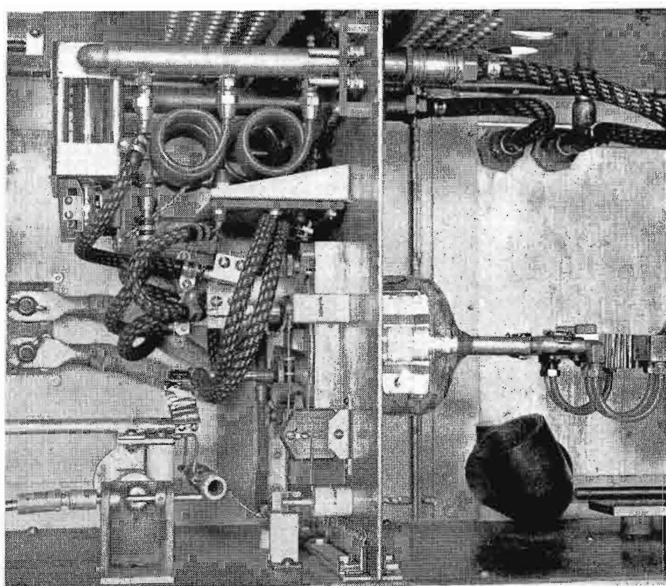
FIG. 5. The 8D21 tube plate in the picture power amplifier section. The Saran insulating coils and water flow interlocks at the top left are permanently mounted on the tube plate.
