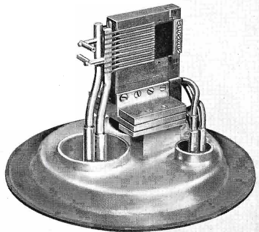
HEADER WITH FILAMENT AND GRID № 1 IN POSITION
