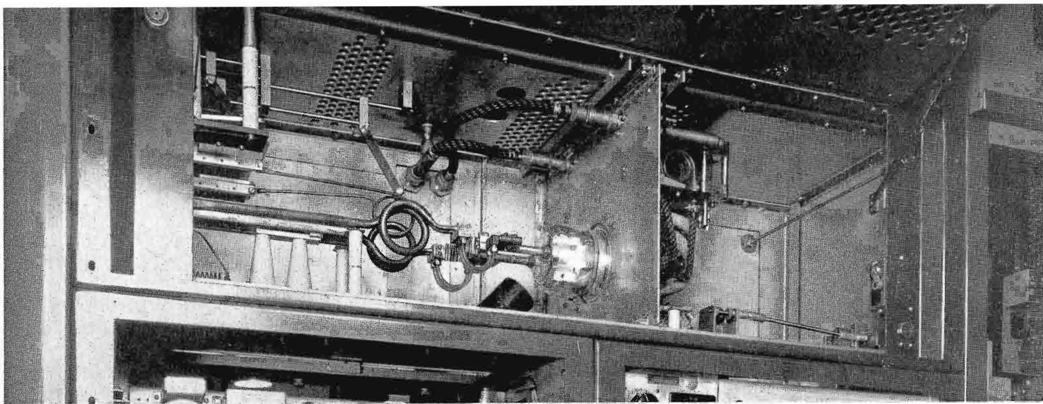
FIG. 4. The sound power amplifier section of the TT-5A with 8D21 tube plate in place and all connections made. Only water connections which must be opened in order to remove the tube plate are the quick-disconnect fasteners on the two flexible leads at the top and the clamp-type connectors on the anodes. All four can be removed in a matter of seconds.
