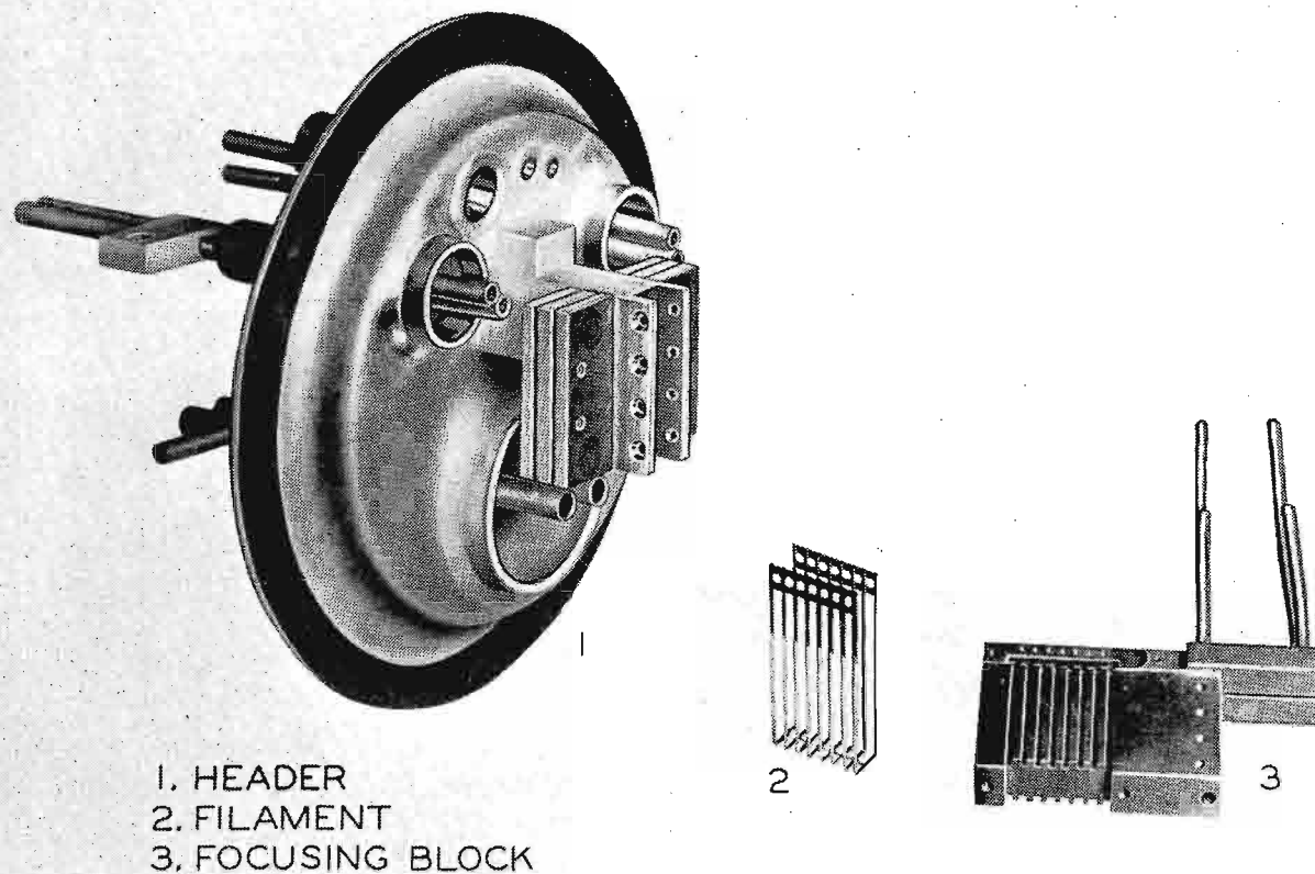
FIG. 3. 8D21 header before assembly. Identified parts are:
