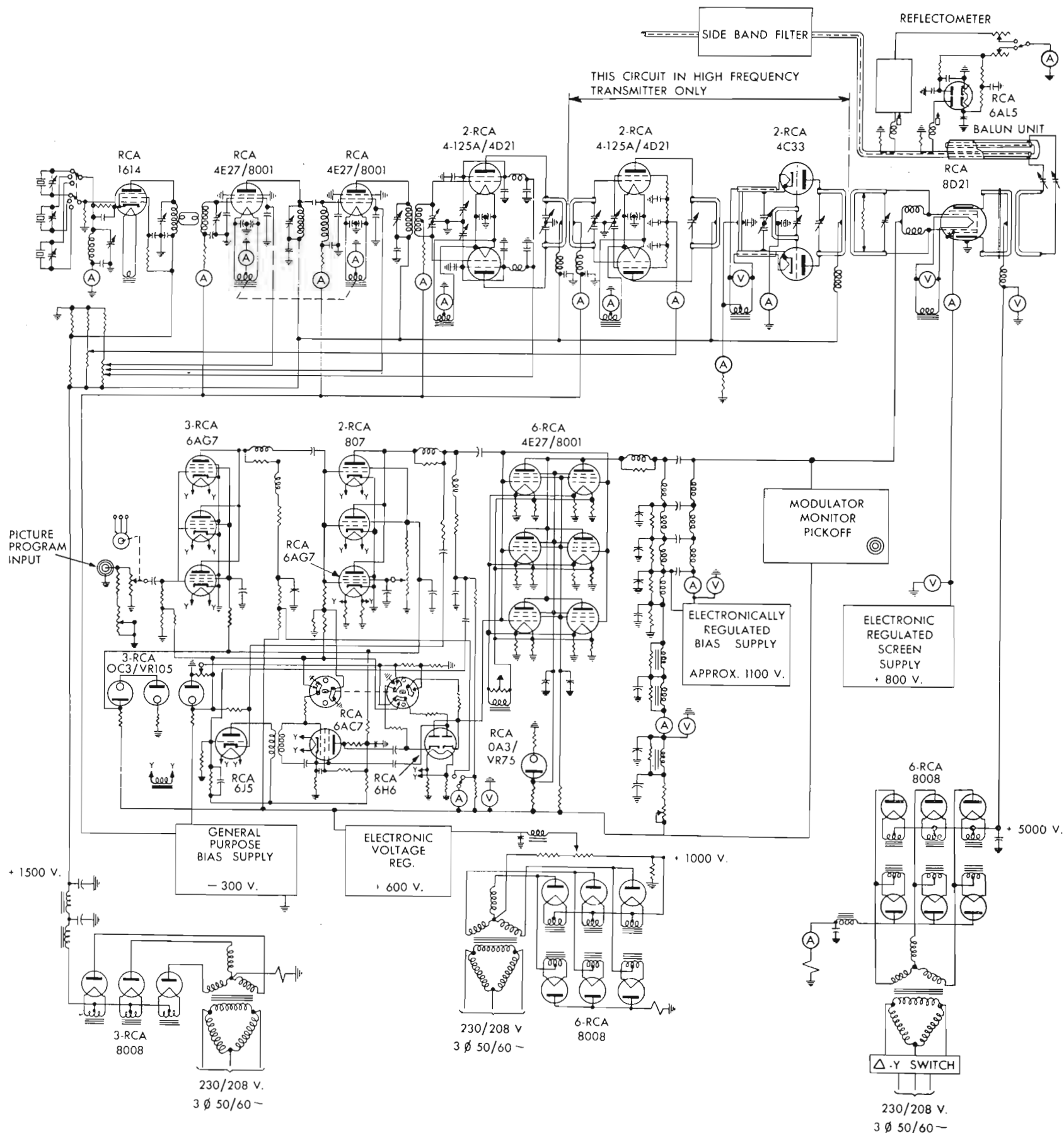
FIG. 4. Schematic diagram of the picture transmitter circuits in the TT-5A equipment. Sound transmitter circuits are shown in diagram of page 10.
