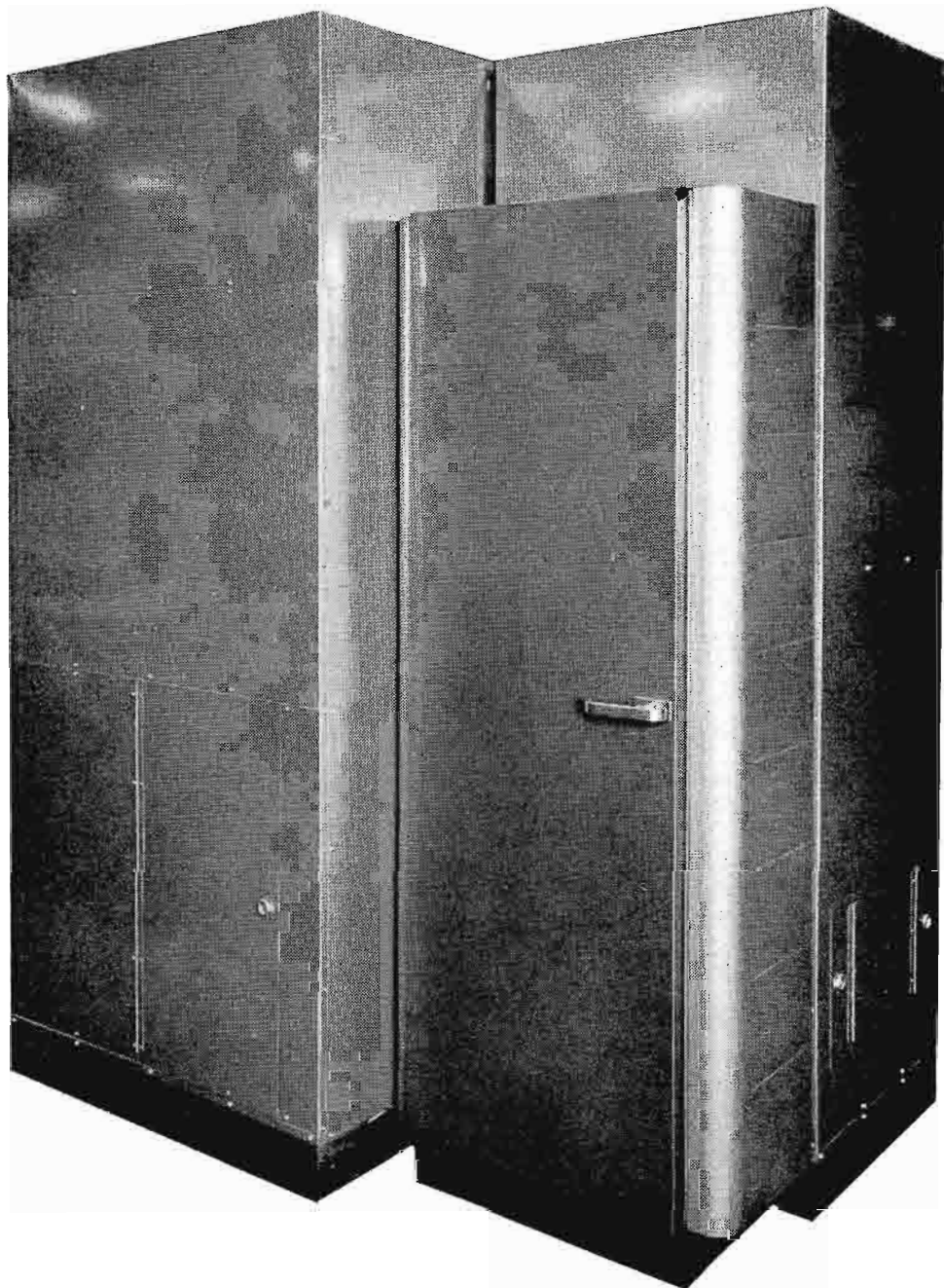
FIG. 11. (above) This assembly includes the dummy load, right front; the diplexer, in the tall narrow cabinet at right rear; and the sideband filter in the large cabinet at the right. All three are fixed-tuned units which once properly installed and tuned, require no further attention.
