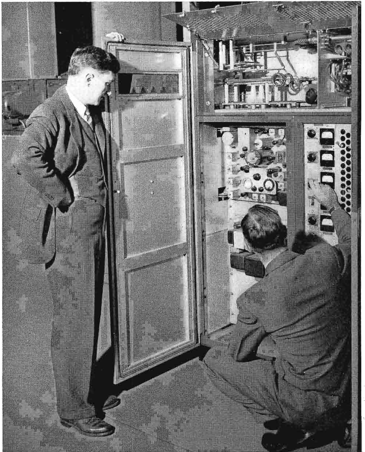
FIG. 10. (right) Open view of frames 1 and 2 containing the sound transmitter. The lower part of frame 1 (left) contains a standard RCA FM exciter unit. The lower part of frame 2 (right) contains the intermediate stages, while the power amplifier is arranged horizontally across the top part of the two frames. In this illustration H. E. Gihring (right), manager of RCA Television Transmitter Engineering Section, explains operation of sound transmitter to Henry Rhea, formerly manager of RCA Television Equipment Sales, now manager of WOWH, Clinton, Illinois.
