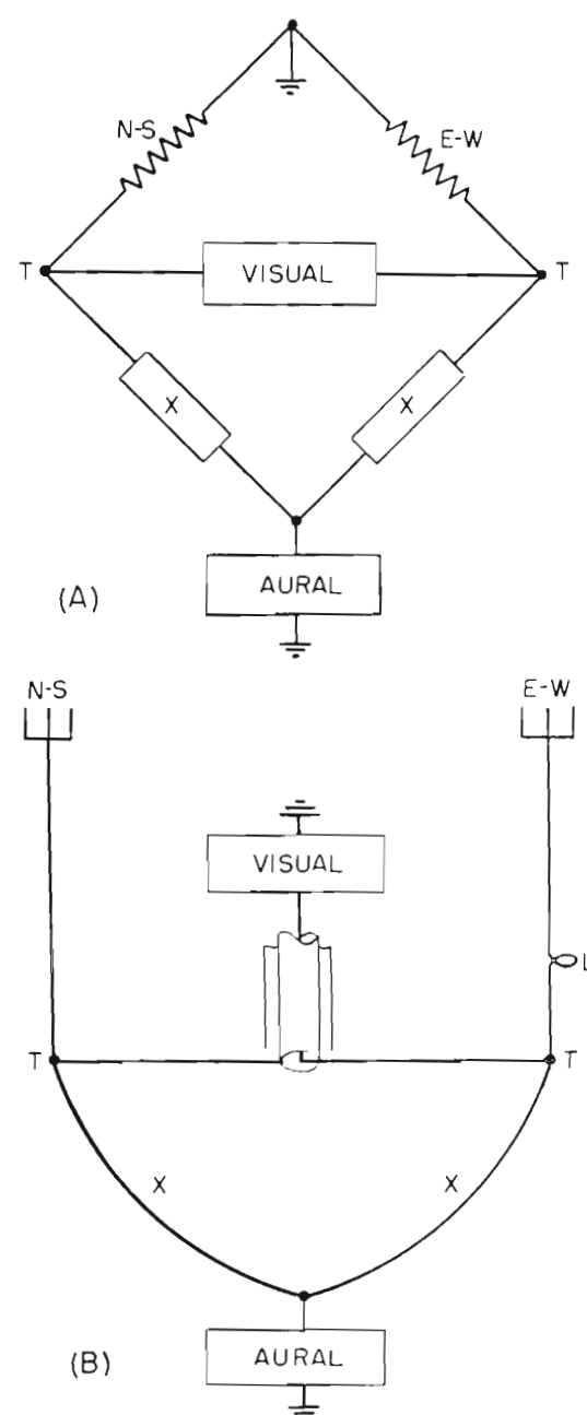
FIG. 4. (right) Fundamental bridge-type diplexing circuit (A) and practical application (B) to visual-aural diplexing system of television transmitter. Circuit lines represent inner conductors of coaxial lines.
