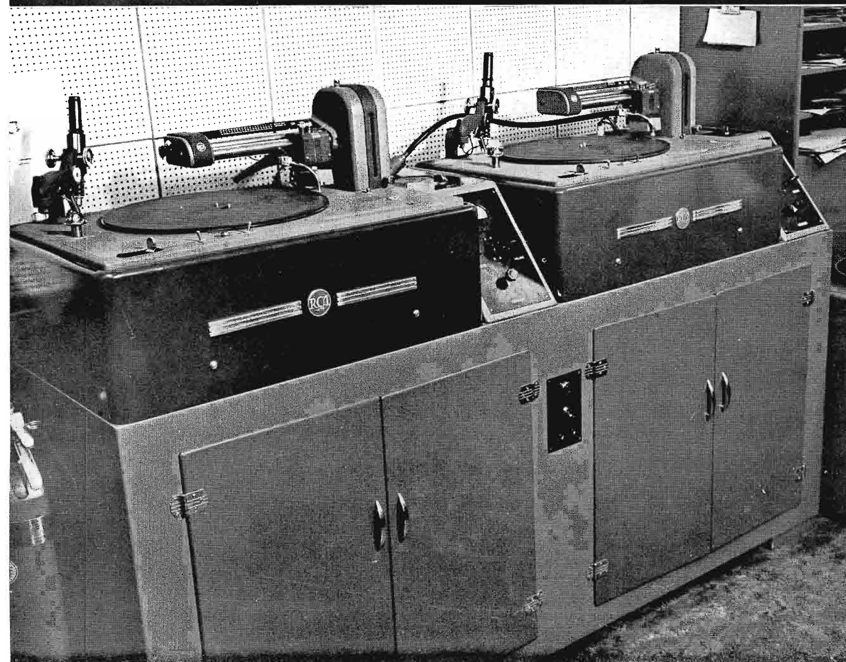
FIG. 2. Closeup view of the recording console at KFBK. At the right of each of the 73-B Recorder units is a sloped panel containing VU meter, start-stop switch, volume control and input line selector switch. Base cabinet, besides acting as mounting for recorder units, provides space for storage of uncut discs and accessory equipment.
